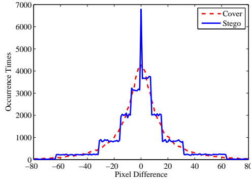
FIGURE 8. The histogram of pixel difference for a cover image and its stego image. The ranges in the stego image are set to as R_1 = [0, 7] , R_2 = [8, 15] , R_3 = [16, 31] , R_4 = [32, 63] , R_5 = [64, 127] , R_6 = [128, 255]
