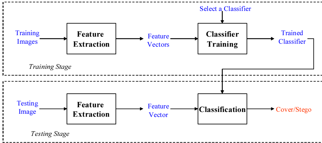
FIGURE 12. The process of a universal steganalytic method
