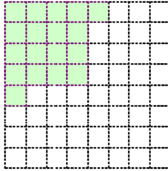
FIGURE 2. Partitioning of the 8×8 DCT coefficient block into two groups for feature extraction
