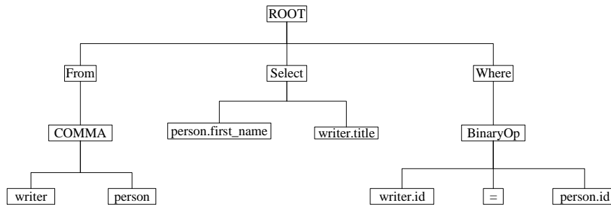
FIGURE 2. The abstract syntax tree of Q_1 .
